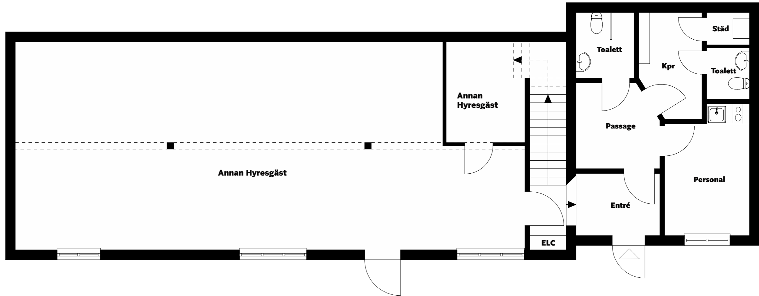
Bottenplan
