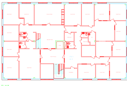
PLAN 2
